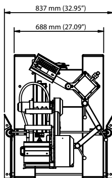
Dimensions refer to 2200 T2200 Long
